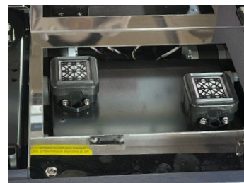
Upgraded Double Head Base Plate
